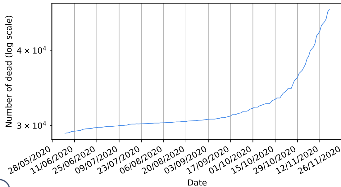
Cumulated number of dead vs date
