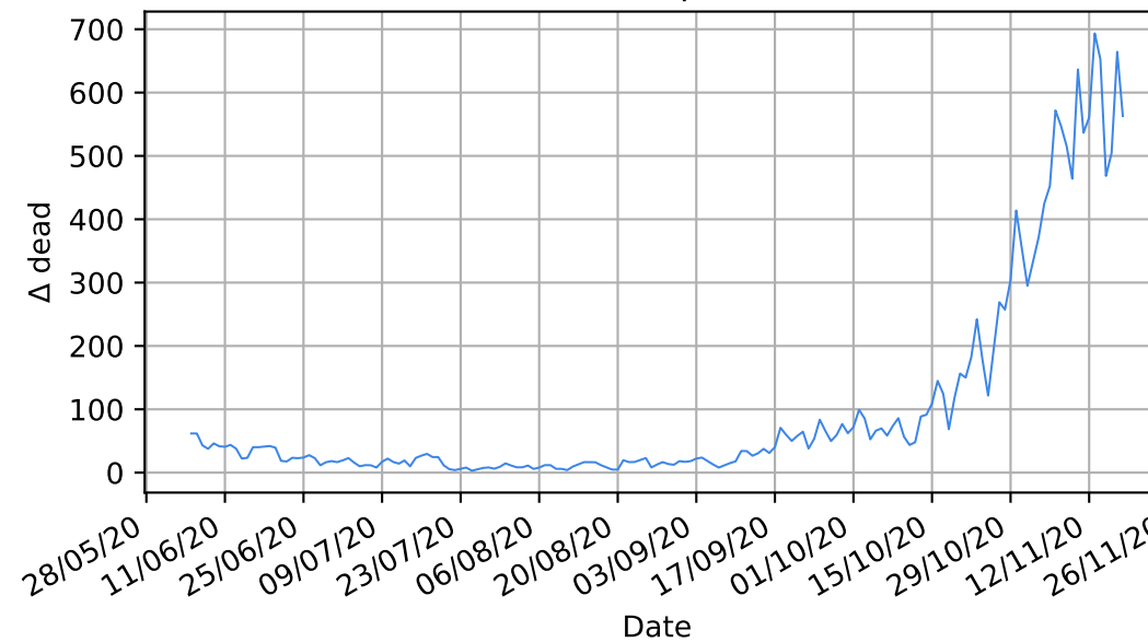
New dead compared to d-1
