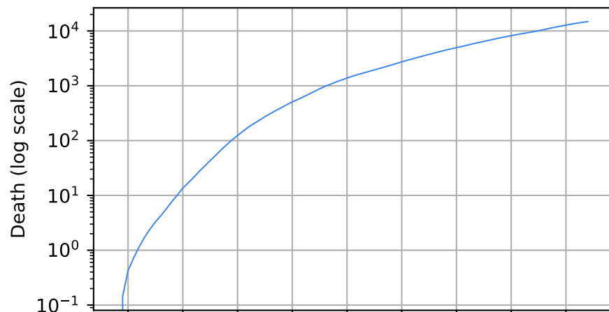
Number of dead
