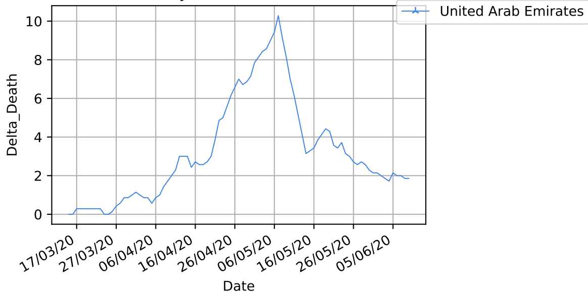
Daily number of death
