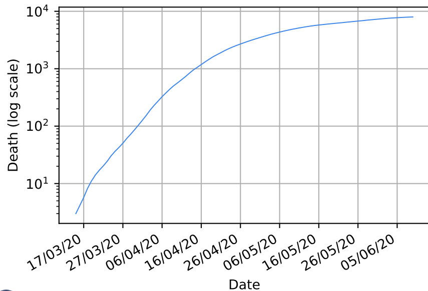
Number of dead
