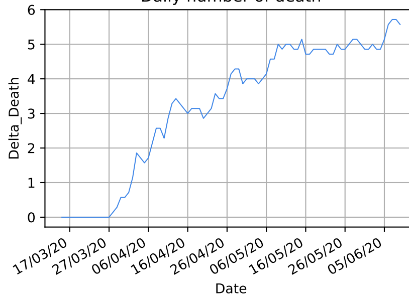
Daily number of death
