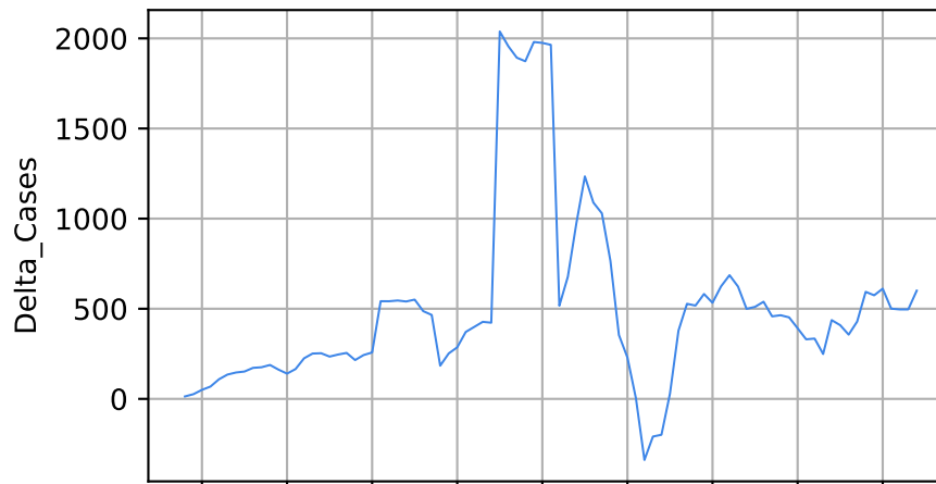
Daily number of cases
